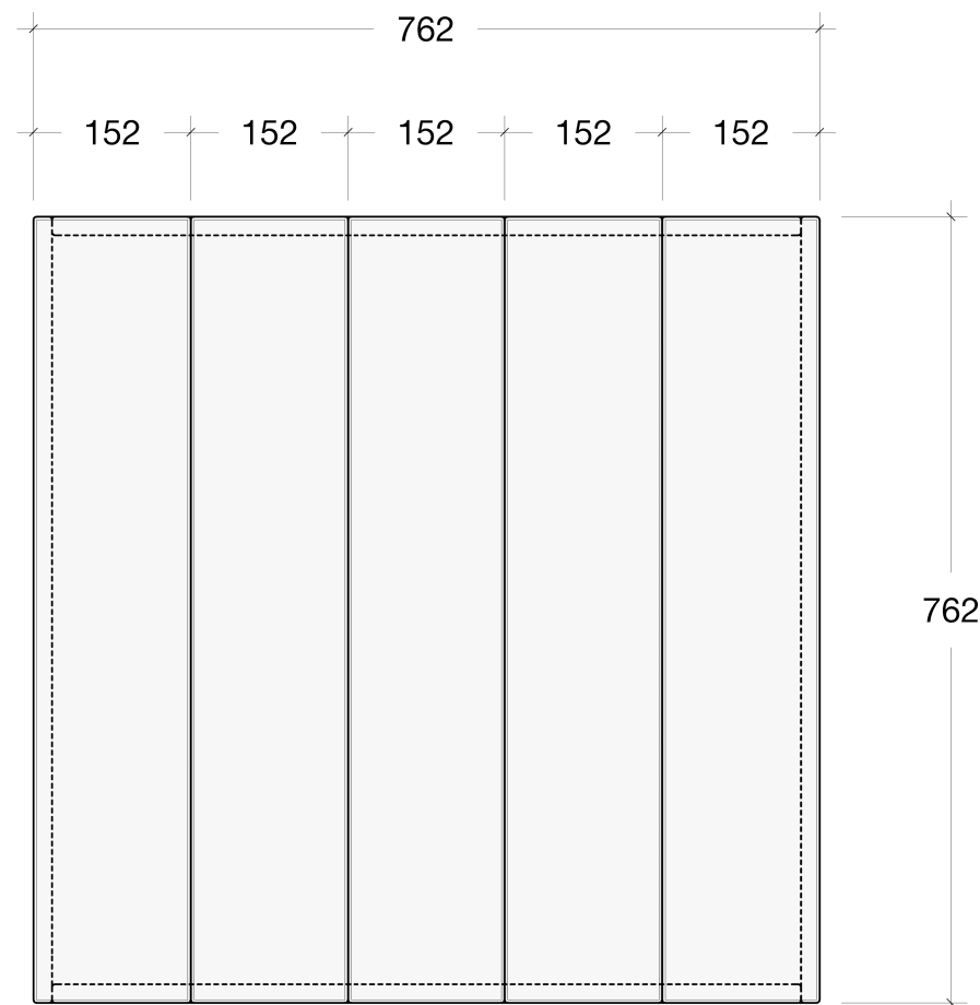
PLAN VIEW 1:8 @ A3
